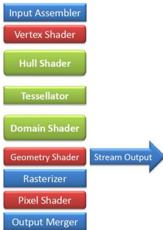
Figure 4 - Shader Model 5.0 Pipeline
