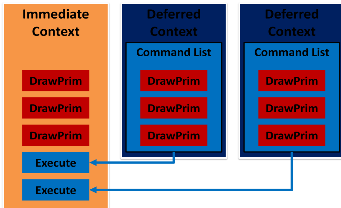
Figure 2 - Direct3D 11 device object contexts
