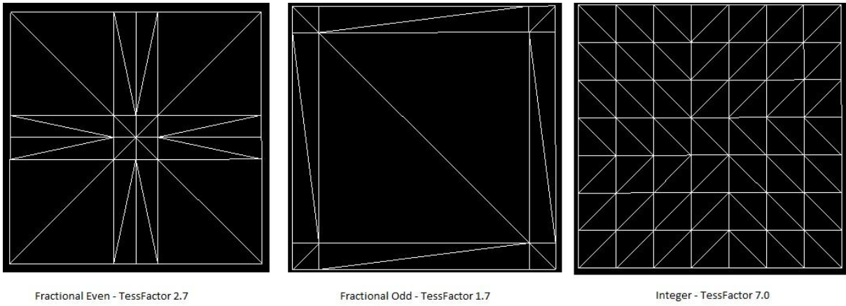
Figure 3 - Tessellation types.
