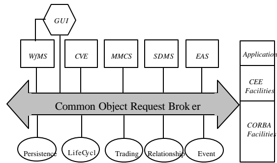
Figure 2: CORBA architecture of the CEE.
